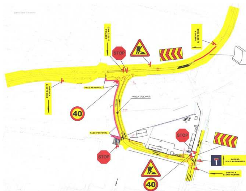
Image 3-28. Detail of diversion in construction work.
