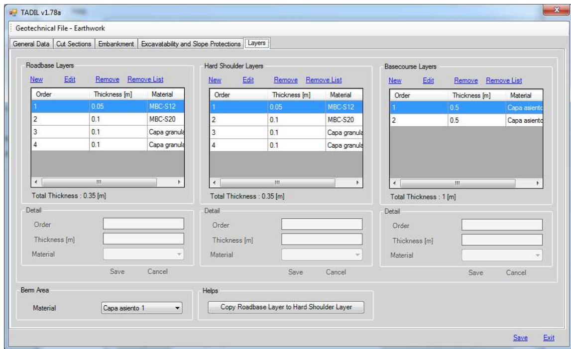
Image 2-7. Input of roadbase layers.
