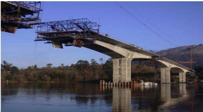
Image 3-15. Bridge post-tensioned on site with variable edge.
